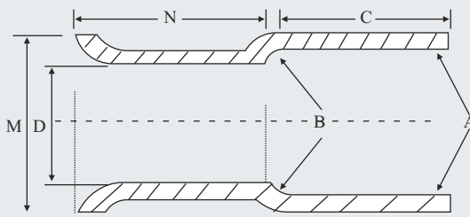
Sizes of couplings and Bell Ends ranges from 1/2", 3/4", 1 1/2", 2", 3", 4", 5", 6", 8", 10", 12", 14", 16"
